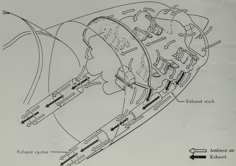
FIGURE 6-37. Engine cooling and exhaust system.
